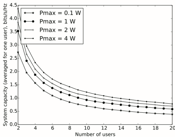
Fig. 6. Average link capacity in the simulated system as function of total number of users
