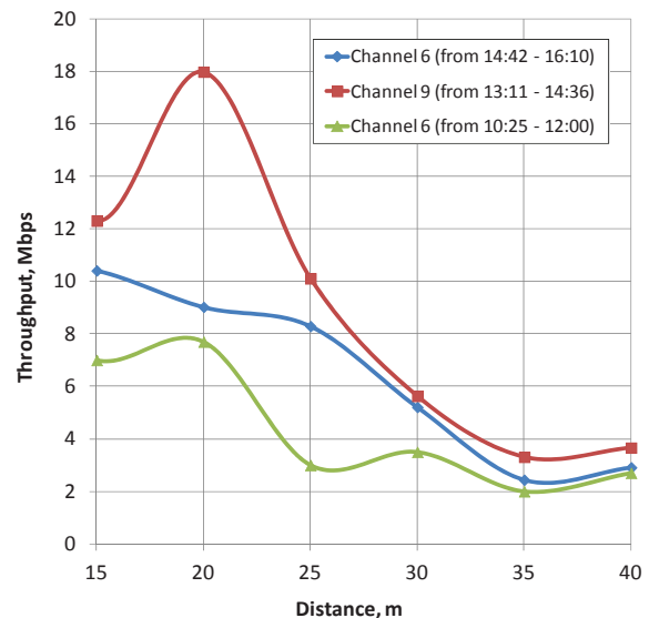
Fig. 1. Throughput of a four-node Wi-Fi IEEE802.11g network as a function of network radius (congested outdoor environment, all terminals at line of sight and RSSI always >-70 dm)
