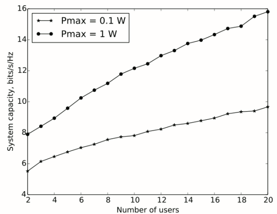
Fig. 4. Total system capacity as function of number of users in a 100x100m area. Simulation results of a distributed interference-aware power control game with the 100mW limit removed, source code available at [52]
